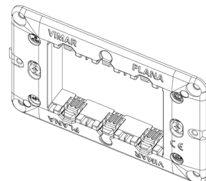
Vista 3D
